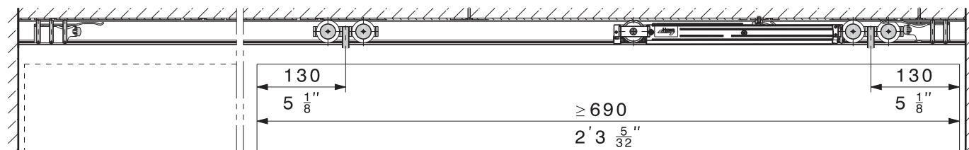
One-sided damping
