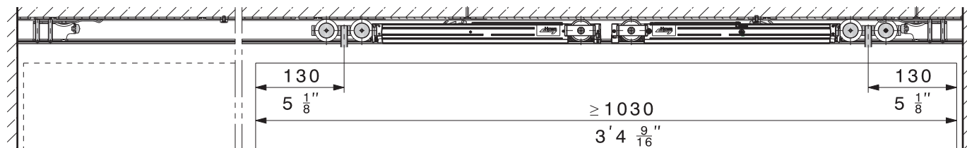
Two-sided damping
